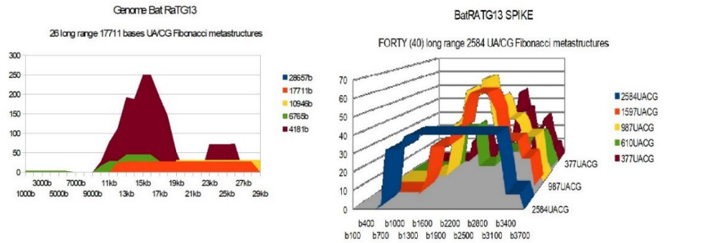
Figure 1 BatRaTG13 Genome and Spike Fibonacci UA/CG metastructures
