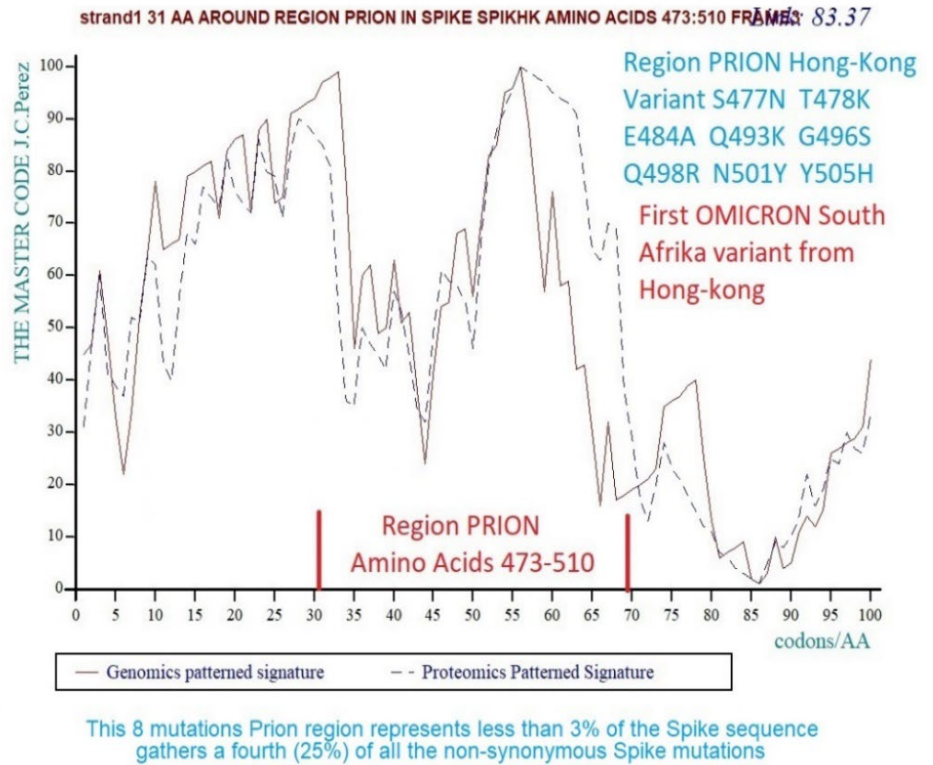
Figure 14 Region PRION in the OMICRON Spike with its 8 amino acids mutations. This is a remarkable observation because this region that represents less than 3% of the spike genome gathers a fourth (25%) of all the Spike non-synonymous mutations
