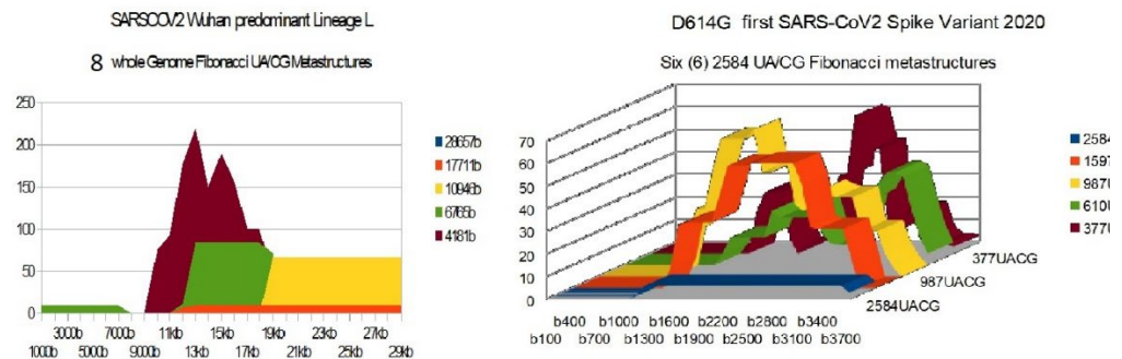
Figure 2 Wuhan lineage L D614G Genome and Spike Fibonacci UA/CG metastructures
