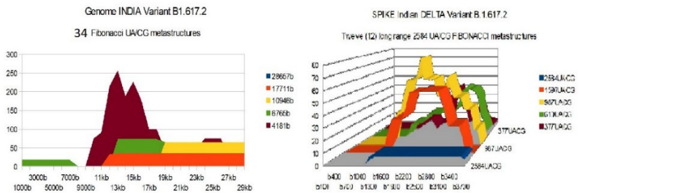
Figure 6 DELTA India B1.617.2 variant Genome and Spike Fibonacci UA/CG metastructures
