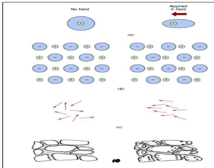
Figure 1: Basic kinds of electric polarization: (a) electronic polarization, (b) atomic or ionic polarization, (c) dipolar polarization and (d) interface or space charge polarization [5].
