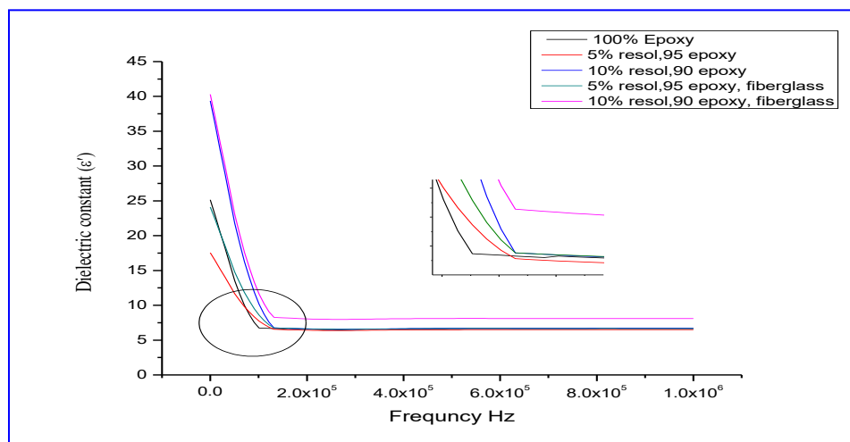
Figure 7: The relationship between dielectric constant and frequency.
