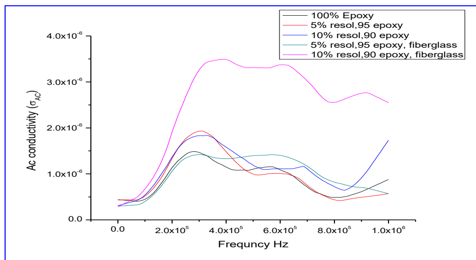
Figure 8: The relationship between A.C conductivity and frequency.
