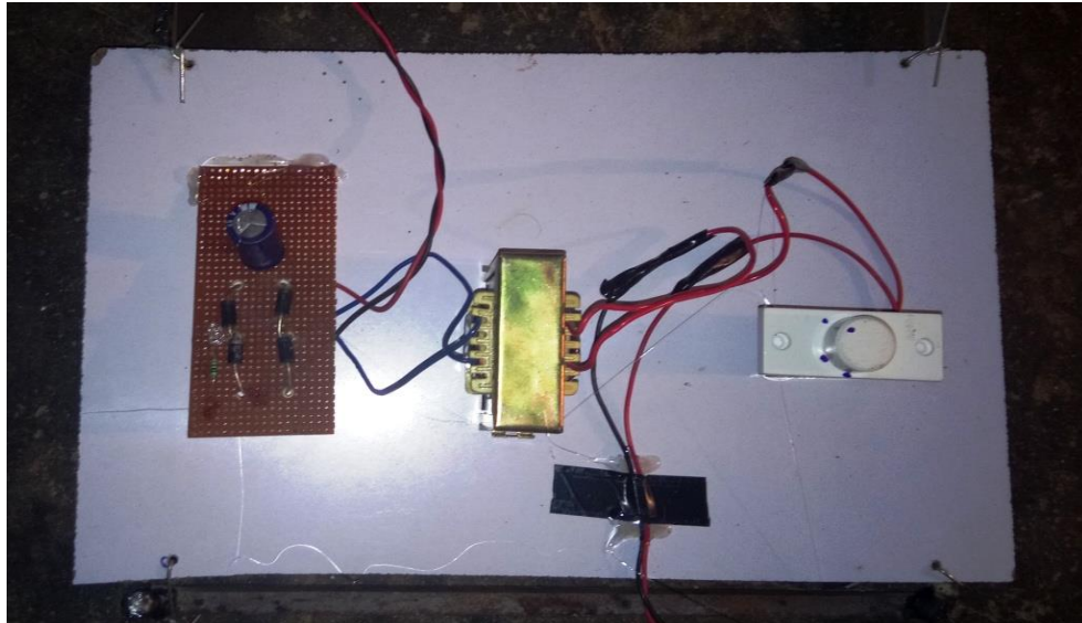
Figure 2: Control Panel
