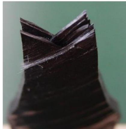
Figure 6: fracture surface of a specimen after tension test (fiber rolling angle is \pm 45^\circ )
