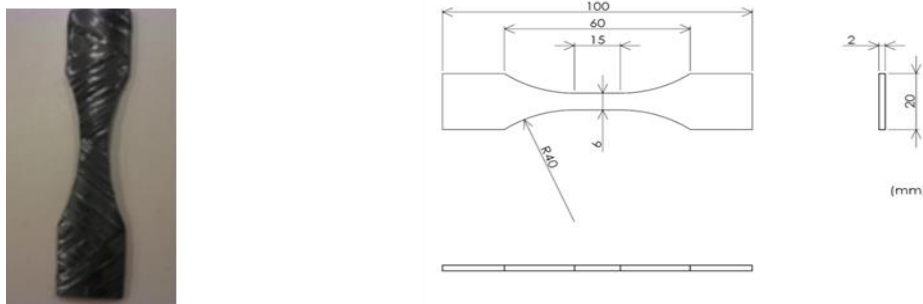
Figure 4: Specimen for a tension test which was cut down from the CFRP circular
