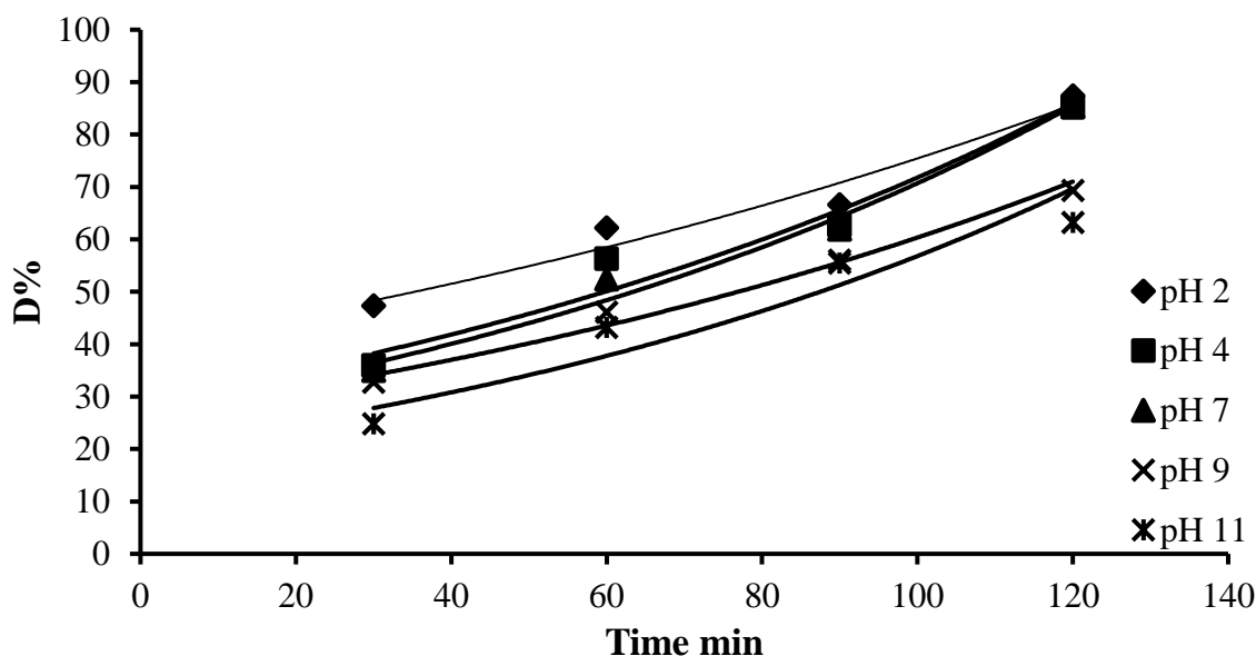
Figure 6: Relation between degradation percent of dye and time by using ZnO, H 2 O 2 at different pH
