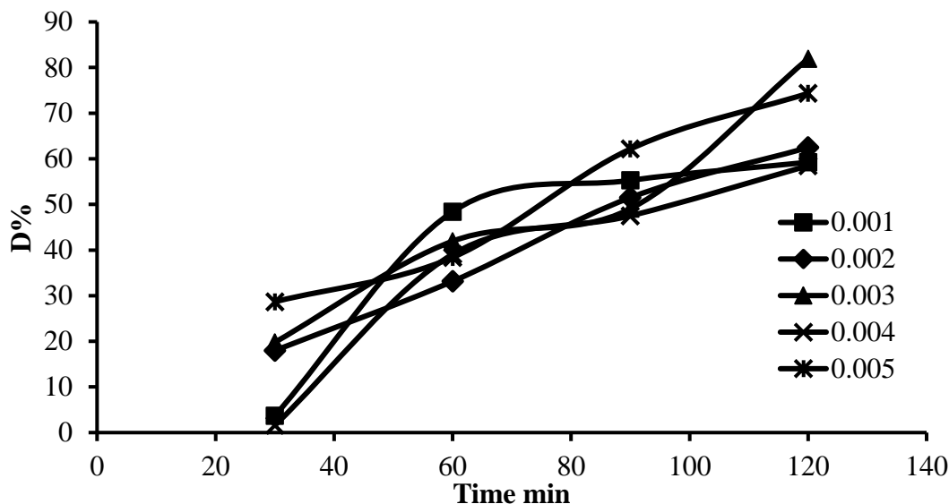
Figure 4: Relationship between the degradation percent of dye against time with using different amounts of catalyst ZnO
