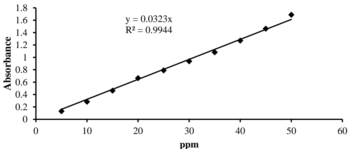
Figure 3: Calibration curve of concentration versus absorbance at 398nm
