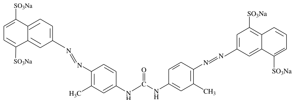
Figure 1: Structure of Direct yellow 50
