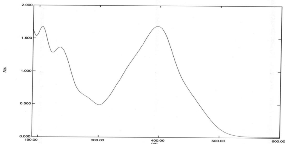
Figure 2: Absorption spectrum of direct yellow 50 in distilled water
