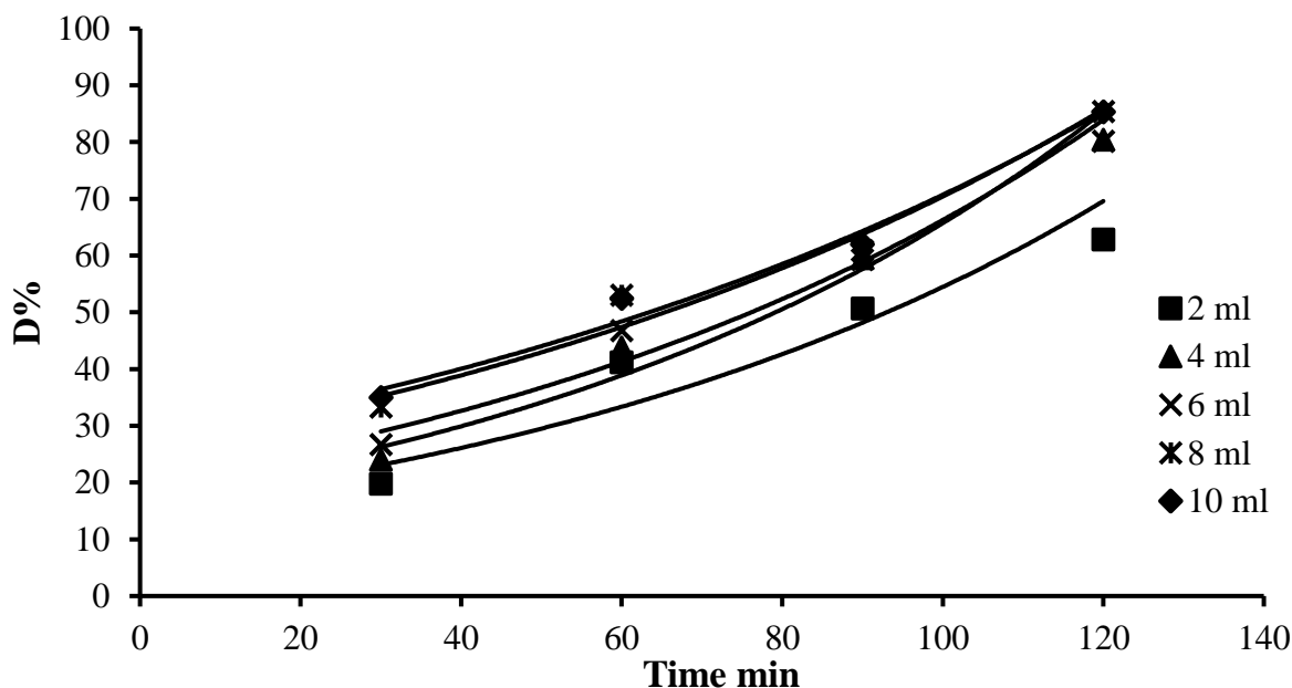
Figure 5: Relation between degradation percent of dye and time by using H_2O_2 as catalysts
