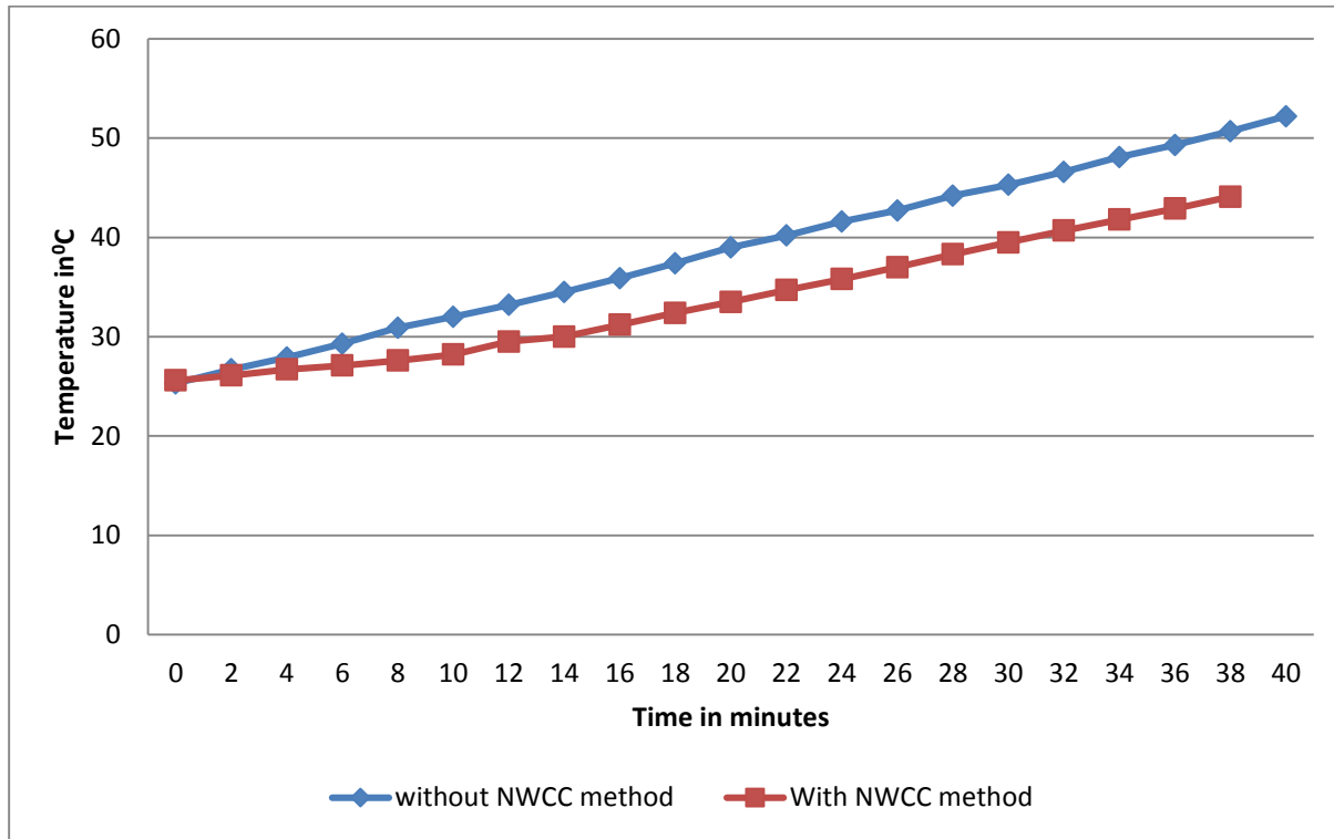
Figure4: Temperature variation of stator with and without NWCC method
