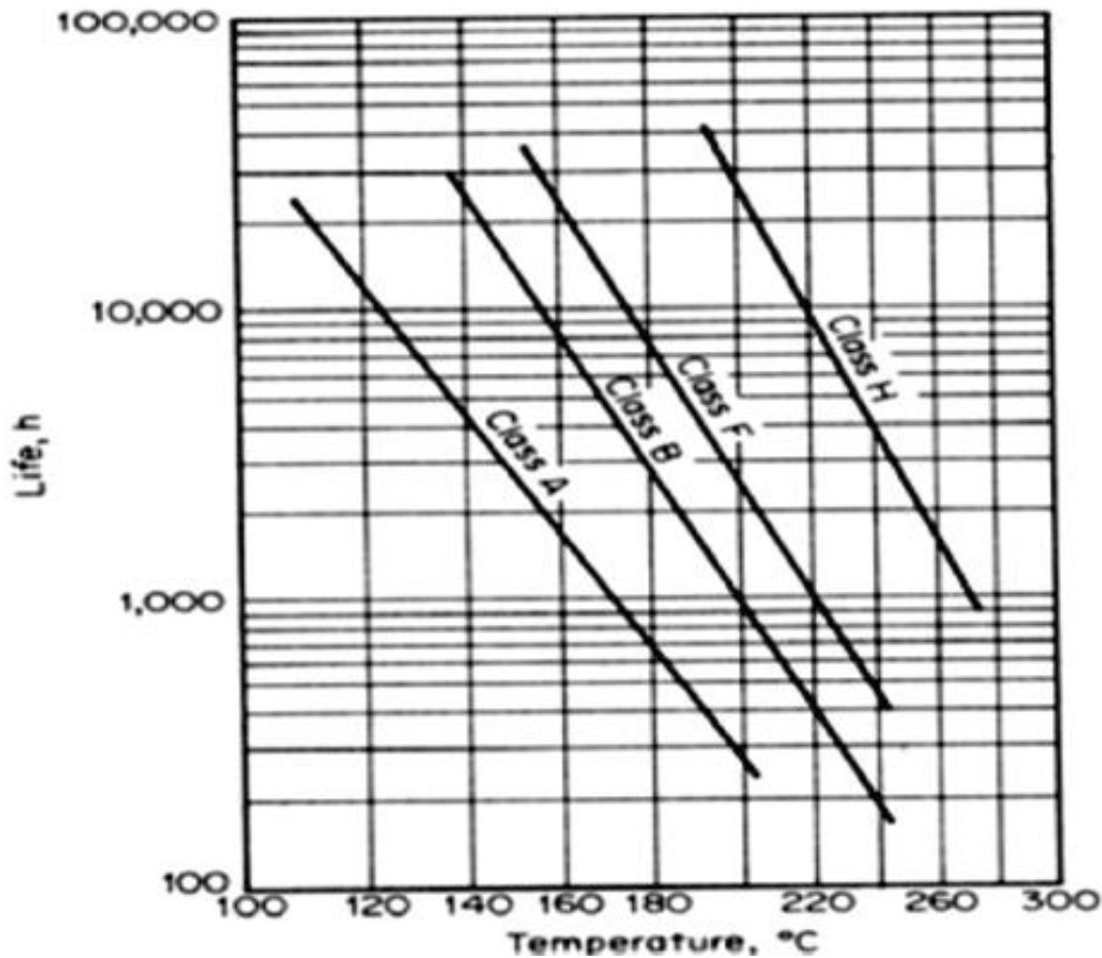
Figure 1. Insulation life versus temperature rise.
