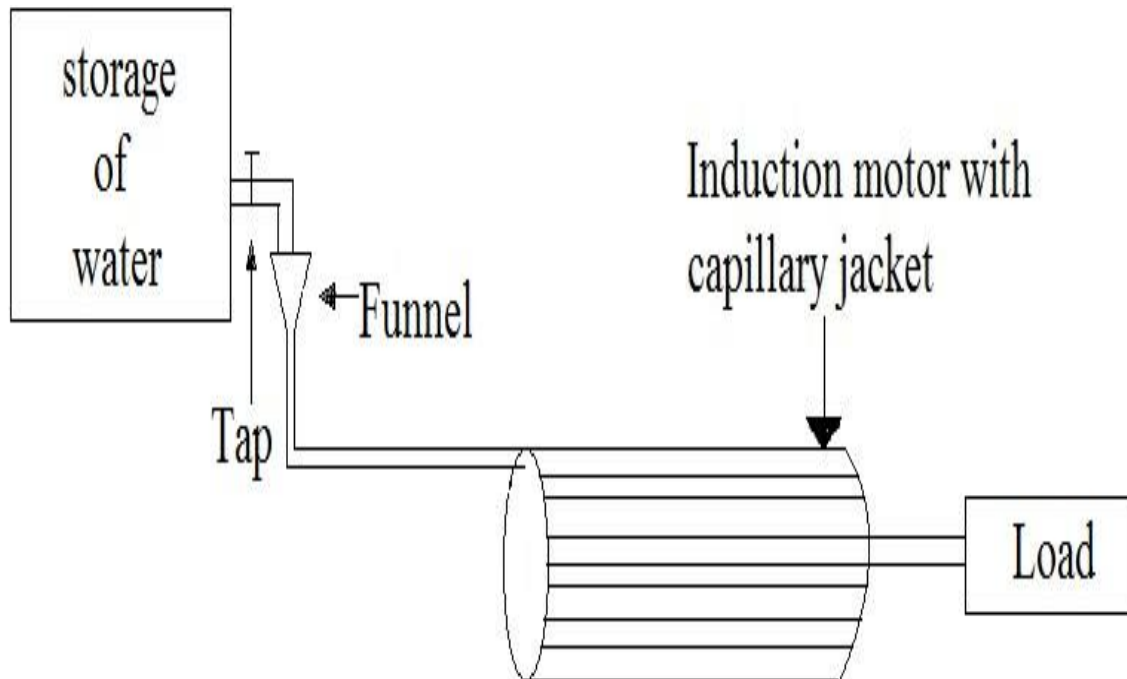
Figure 3: working of NWCC method
