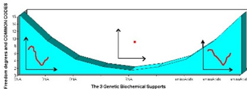
Figure 4 A symbolic representation of the 3 worlds of double stranded DNA (Genomics) highly correlated with potential double stranded amino acids (Proteomics) while RNA double stranded image is like a neutral element.
