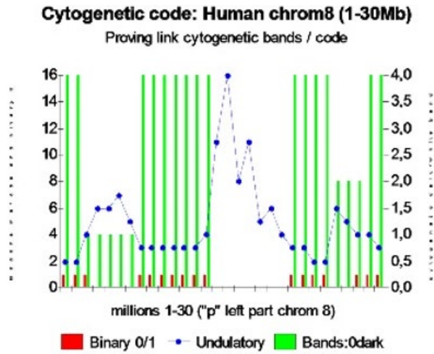
Figure 13 Example of chromosome 8 bands evidence from Proteomics Binary code and Genomics undulatory code (30 first millions bases in human chromosome 8).
