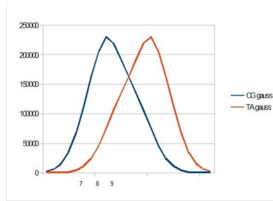
Figure 20 Gauss like CG / TA distribution within the whole human HG38 chromosome21
