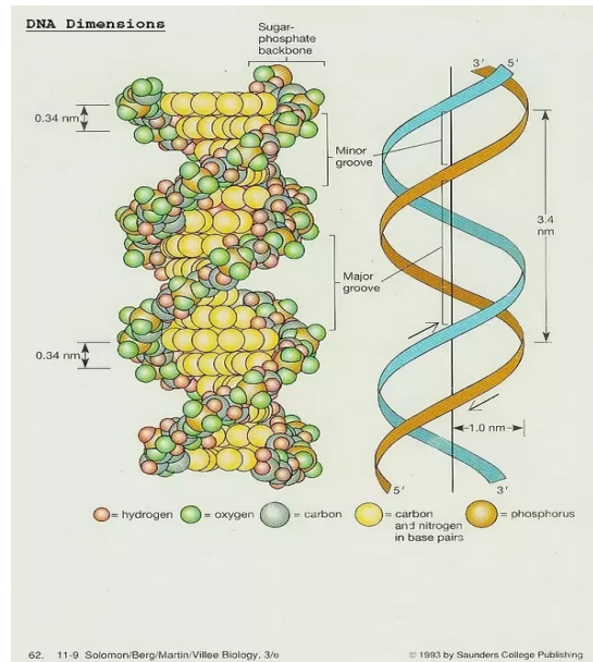
Figure 41 Each DNA helix rises about 34 angstroms during each complete turn
