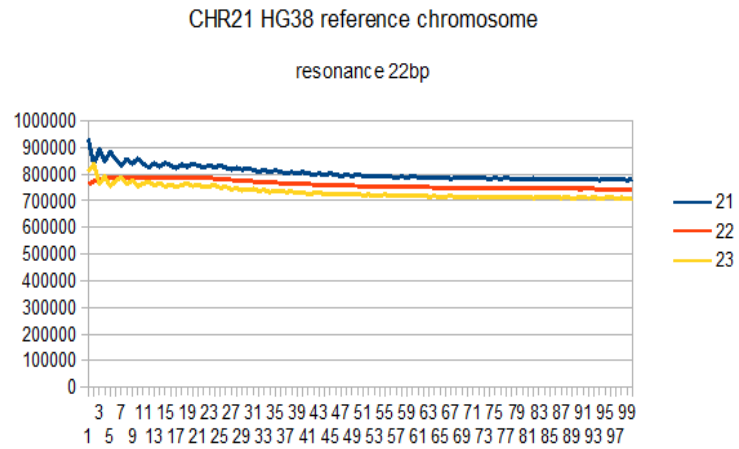
Figure 18 Evidence of a resonance of 22bp period in the whole HG38 human reference chromosome21 (horizontal undulatory code -IV-).
