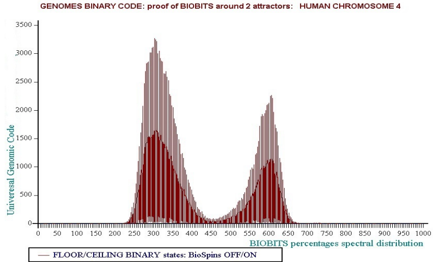
Figure 10 whole chromosome 4 – evidence of the perfect Proteomics Binary Code.
