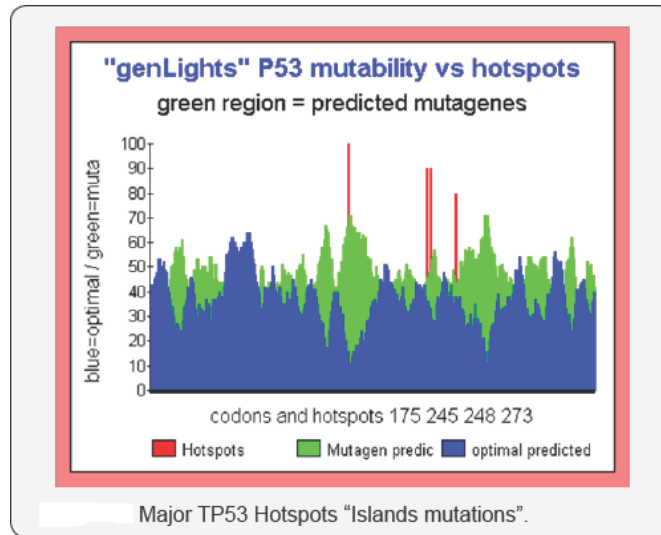
Figure 39 Predicting individual codons mutability potential in TP53 tumor suppressor
