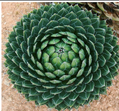
Figure 43 Fibonacci patterns emerging from plant Agave-victoriae-reginae
