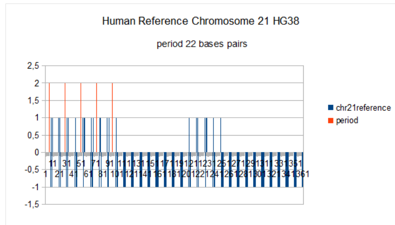
Figure 19 Confirmation of a 22bp period in the whole HG38 human reference chromosome21 - vertical genomic binary code -III-).
