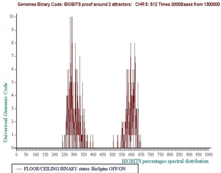
Figure 22 Level 2: 512 times 2000 bases... Consensus Decision "VOTE" = Floor = "False"
