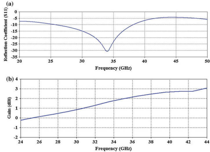
Figure 42 Evidence of a standing wave of 34 Giga Hertz in a modelized DNA molecule using biomaterials (source publication [ Perez (2009) ])
