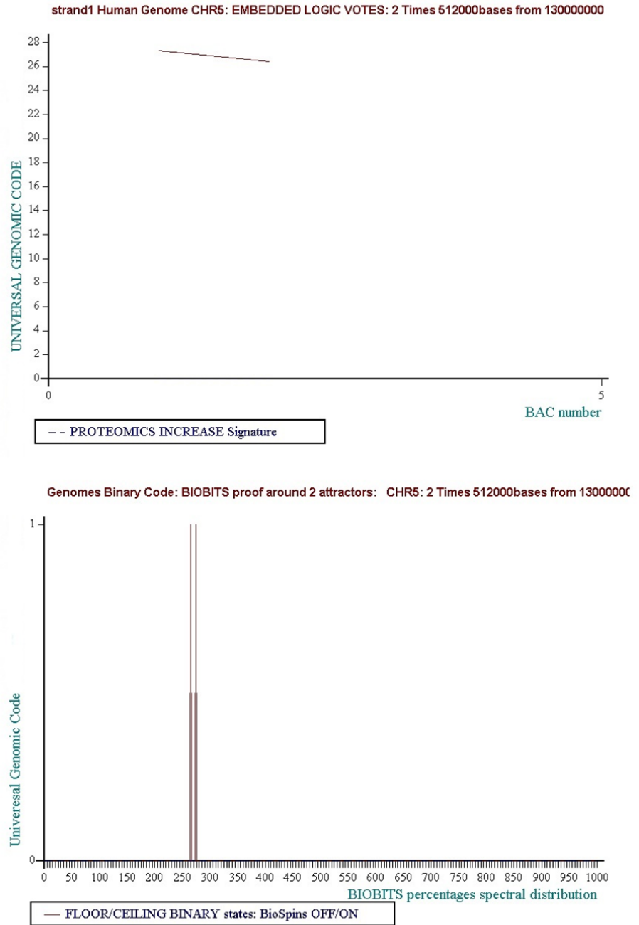
Figure 30 Level 10: 2 times 512000 bases... Consensus Decision "VOTE" = Floor = "False"
