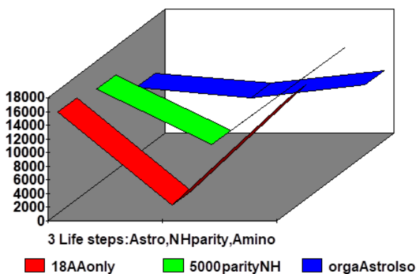
Figure 36 The triple curve in "V", concentrated comparison of lines 4, 6 and 12 of Table 8.
