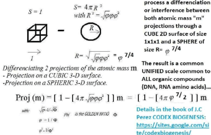
Figure 2 geometric meaning of the formula for life numerical projection
