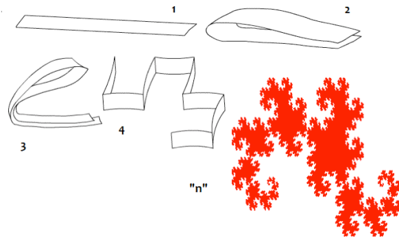
Figure 44 The Fractal "Dragon Curve" manage billions populations of triplets codons in the whole Human Genome
