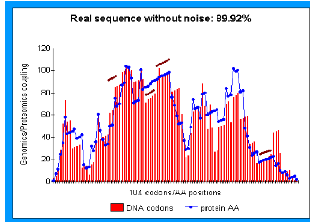
Figure 7 Evidence of first-order differential texture and roughness analysis (Leibniz) on Master Code Genomics and Proteomics images.
