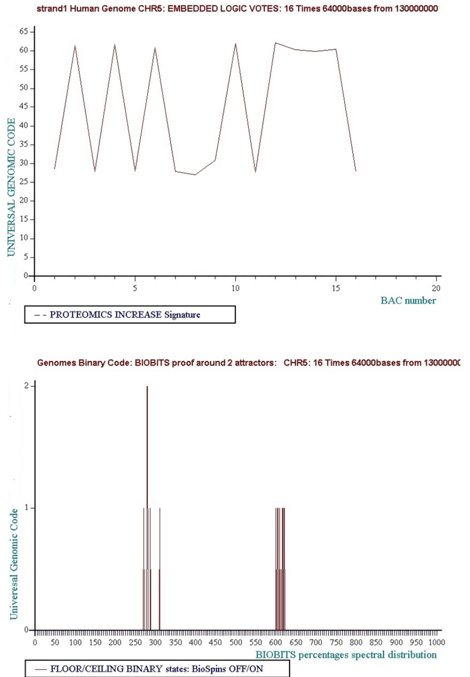
Figure 27 Level 7: 16 times 64000 bases... Consensus Decision "VOTE" = "Undefined"
