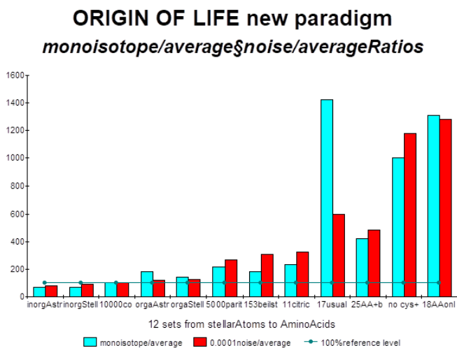
Figure 35 The comparison of the ratios "monoisotopic mass / average mass" between real cases and noisy cases.
