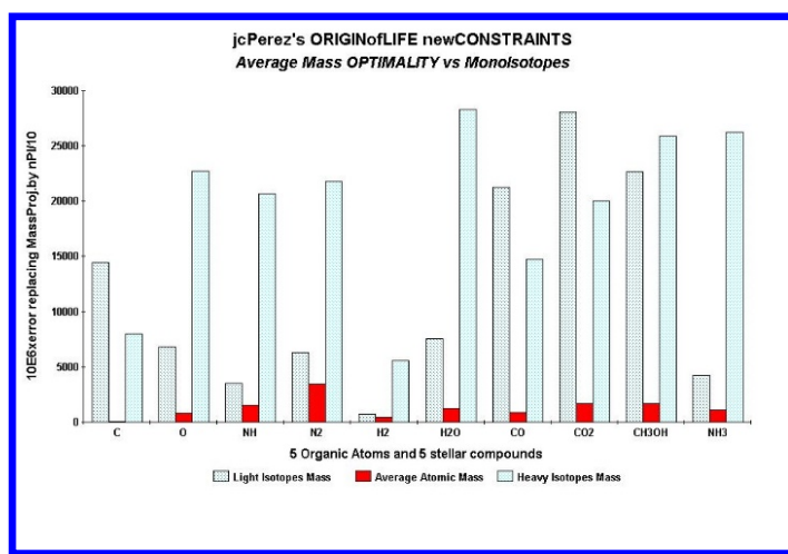
Figure 33 The OPTIMALITY of the average atomic mass is proved here on the PI-masses of ten primordial organic components.
