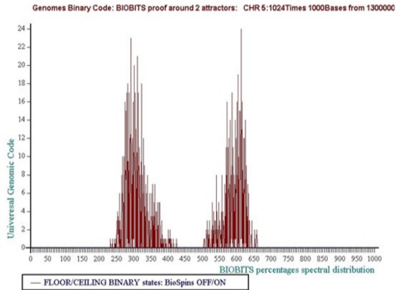
Figure 21 Level 1: 1024 times 1000 bases... Consensus Decision "VOTE" = Floor = "False"
