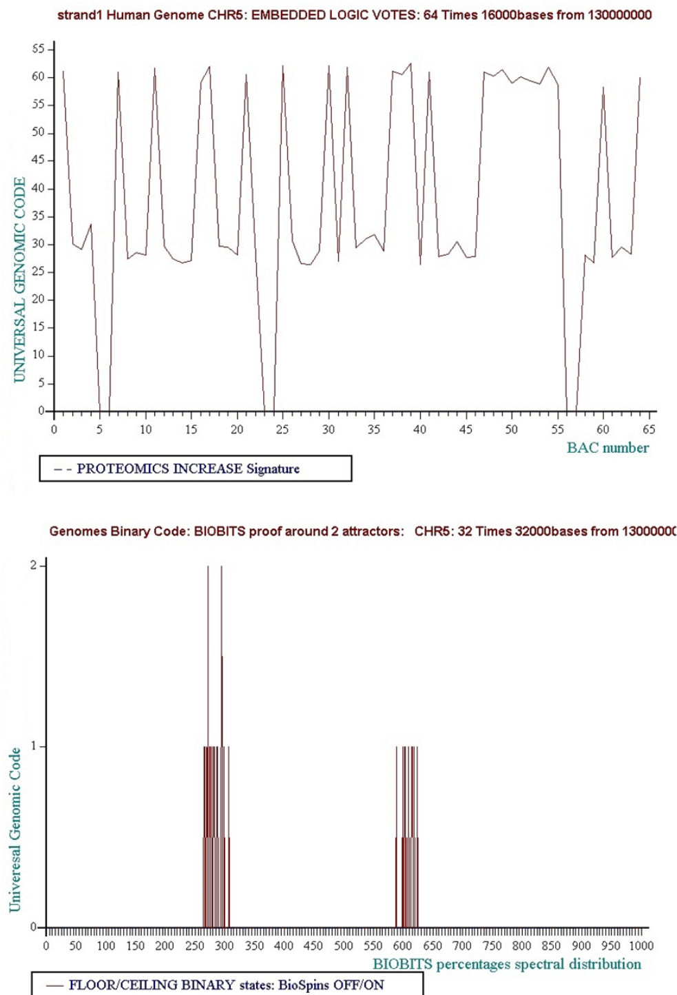
Figure 26 Level 6: 32 times 32000 bases... Consensus Decision "VOTE" = Floor = "False"
