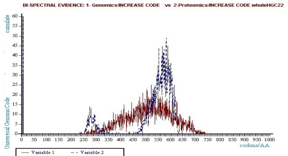
Figure 9 Frequency distribution - In whole chromosome 22, population of Genomics curves will be relatively dispersed around one single withdrawing attractor in a kind of Gaussian dispersion (red), while the population of Proteomic curves will be distributed around two binary attractors (blue).
