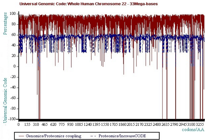
Figure 8 Clouds of points - In whole chromosome 22, population of Genomics curves will be relatively dispersed around one single withdrawing attractor in a kind of Gaussian dispersion (red), while the population of Proteomic curves will be distributed around two binary attractors (blue).
