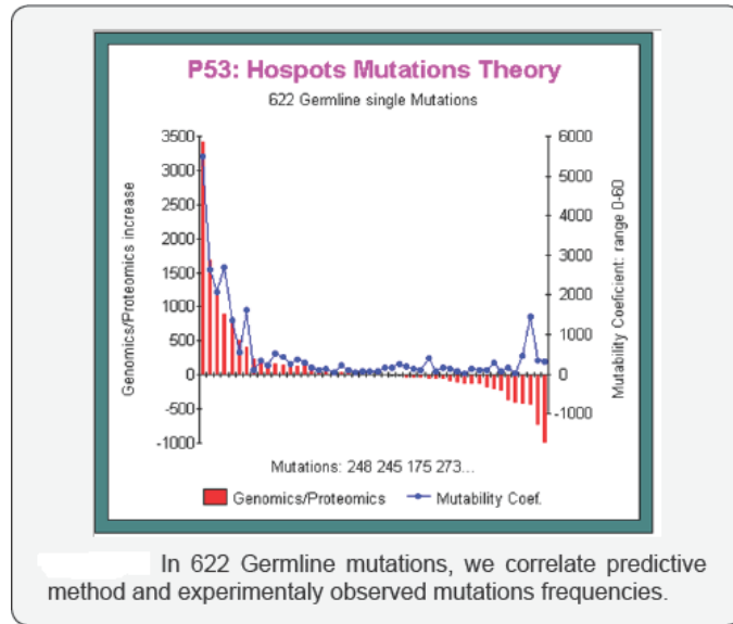
Figure 38 In 622 Germline mutations, we correlate predictive method and experimentally observed mutations frequencies.
