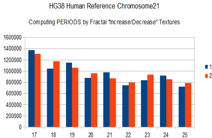
Figure 17 zoom on vertical scan method revealing PERIOD = 22 from HG38 reference chromosome21.
