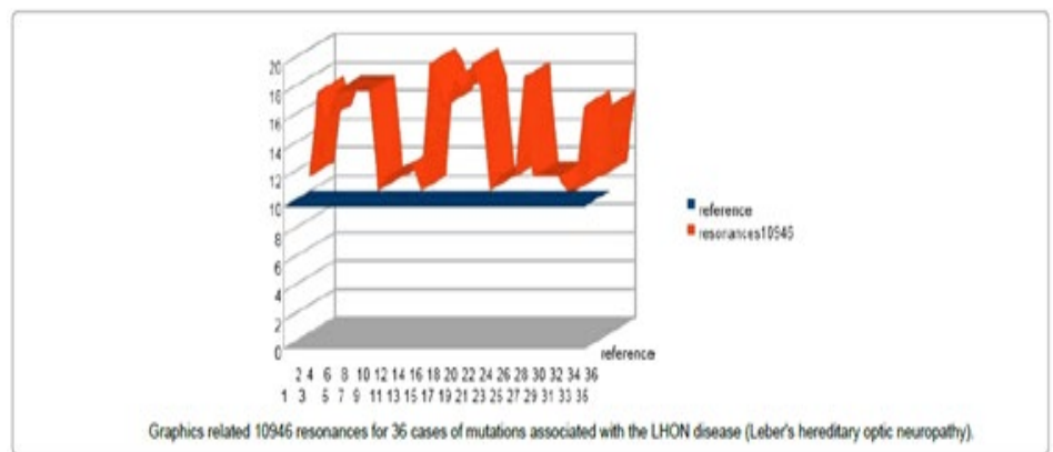
Figure 37 Graphics related 10946 resonances for 36 cases of mutations associated with the LHON disease (Leber's hereditary optic neuropathy). In this figure, the 36 LHON mutations on mtDNA genome INCREASES the number of long 10946 Fibonacci “resonances”.
