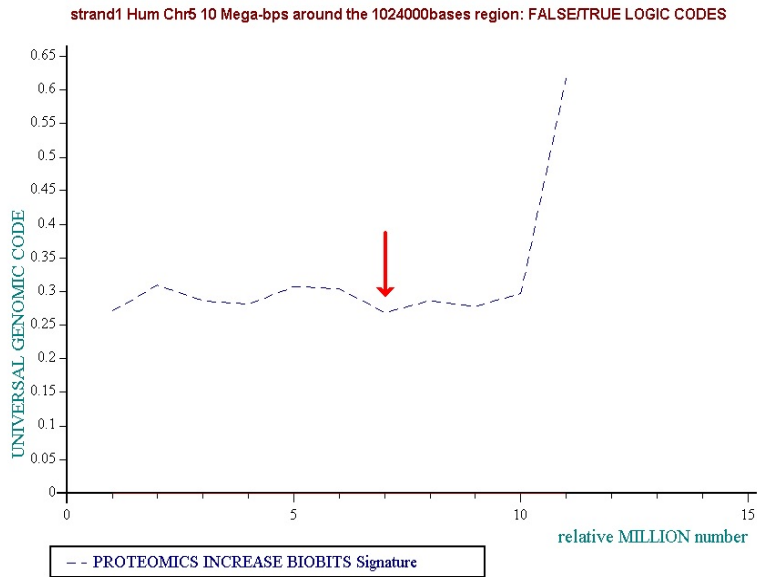
Figure 31 10 millions bases genomic region around the 1024000 bases analysed region is globally also in “floor” binary state.
