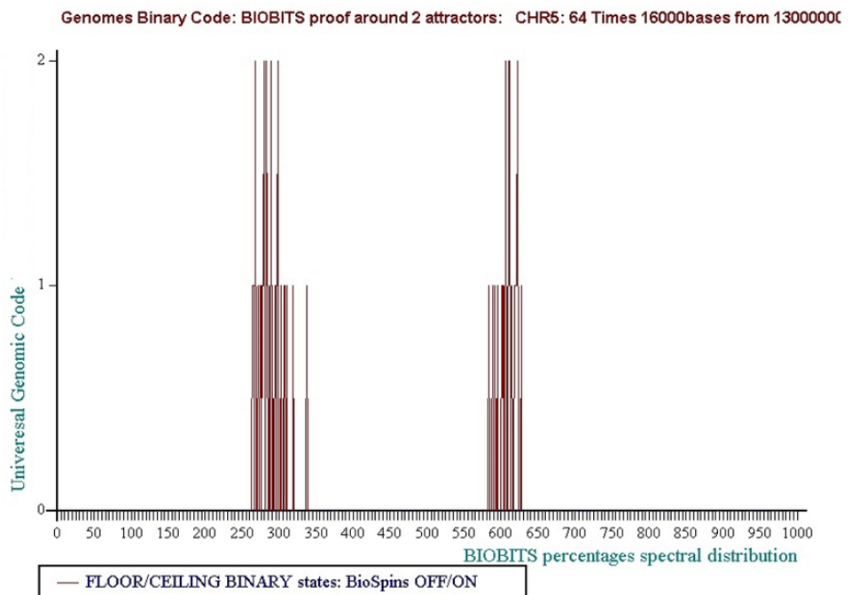
Figure 25 Level 5: 64 times 16000 bases... Consensus Decision "VOTE" = Floor = "False"
