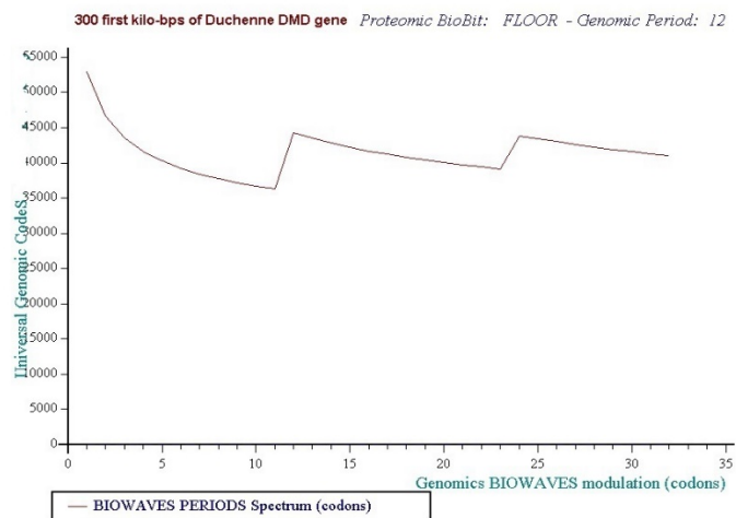
Figure 12 Long waves from Genomics master code images (300000 bases from DMG gene (Duchenne Muscular Distrophy)).
