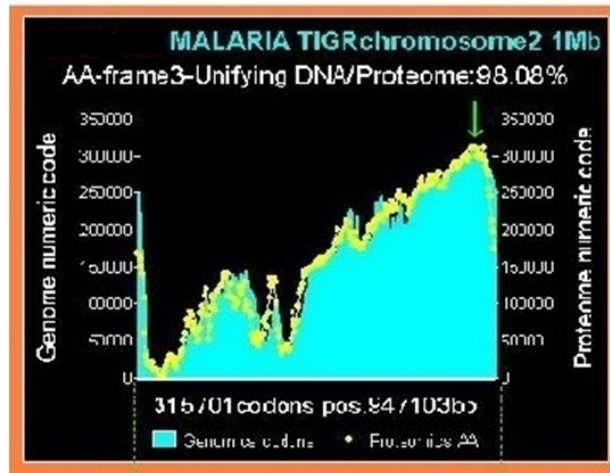
Figure 6 illustration of the high correlation coupling between genomics and proteomics images of a complete MALARIA chromosome (98.08% correlation).
