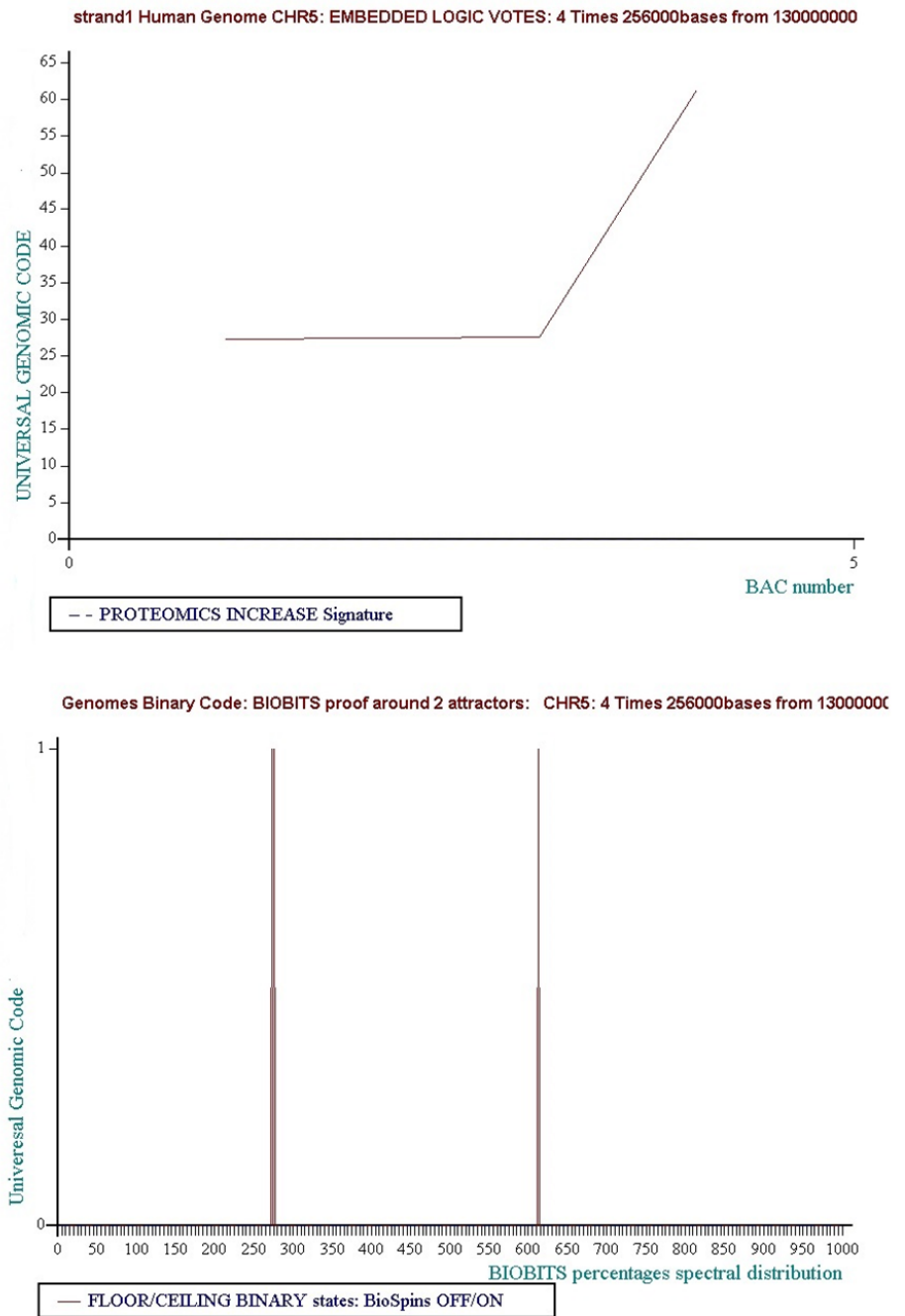
Figure 29 Level 9: 4 times 256000 bases... Consensus Decision "VOTE" = Floor = "False"
