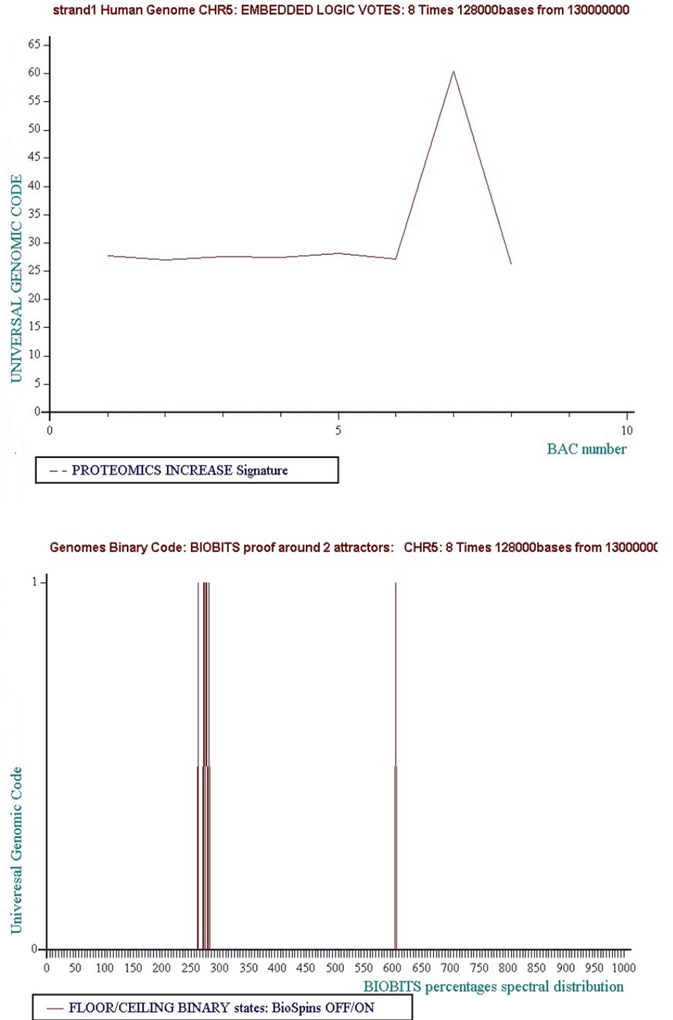
Figure 28 Level 8: 8 times 128000 bases... Consensus Decision "VOTE" = Floor = "False"
