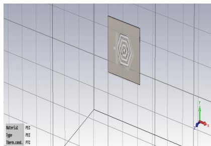
Figure 2: Back side of proposed moisture sensor
