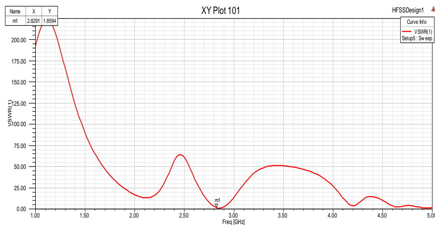
Figure 4: VSWR of Antenna
