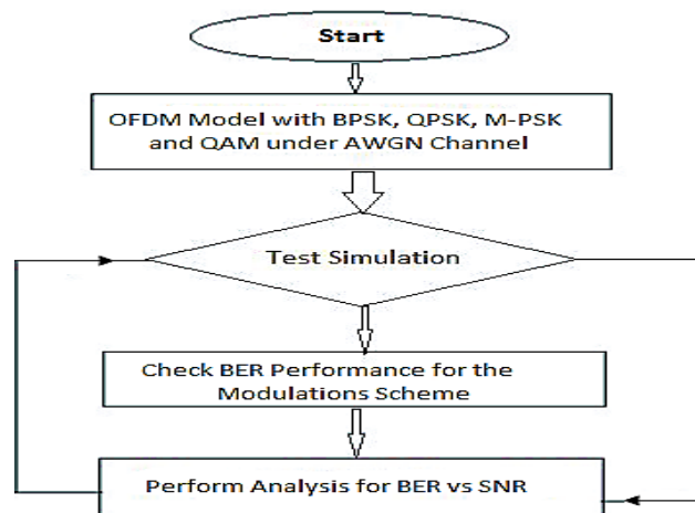
Figure 6: Flow Chart
