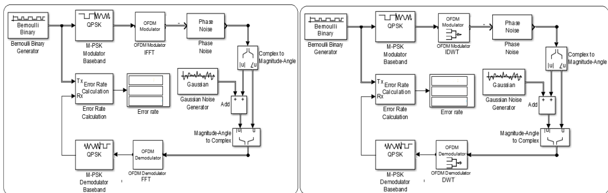
Figure 2: Simplified OFDM Simulink Model for DWT and FFT [5]
