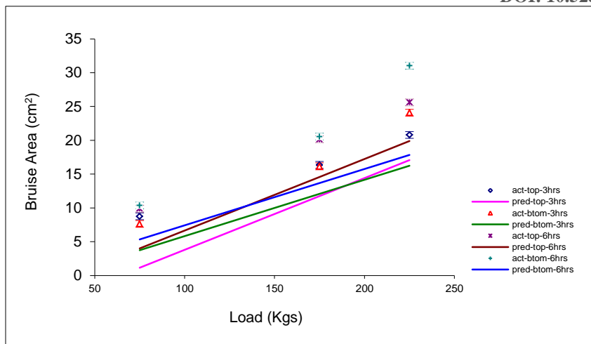
Figure 7: Plot of actual average bruise area and predicted bruise area based on the models for Mat1 nuts
