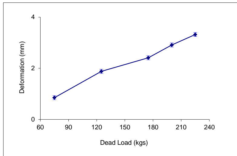
Figure 5: Effect of load on deformation
