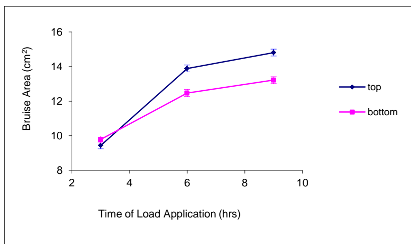
Figure 2: Effect of time of load application on bruise area
