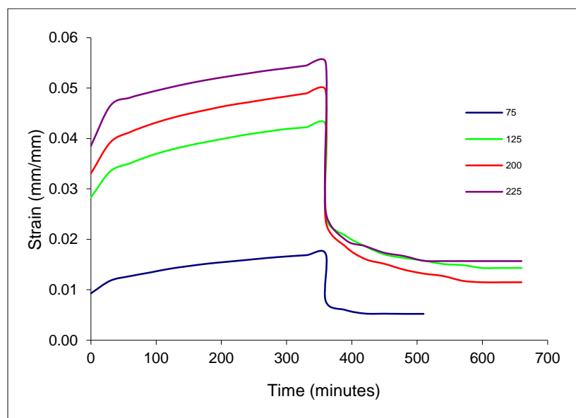
Figure 6: Creep and recovery curves for young coconut
